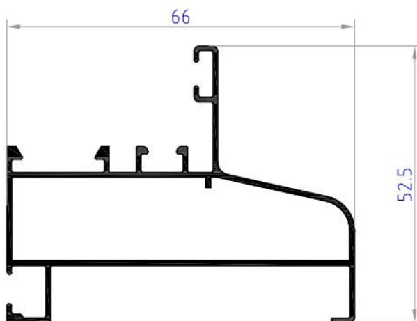
PS6648 weight 0.610 kg/ml
