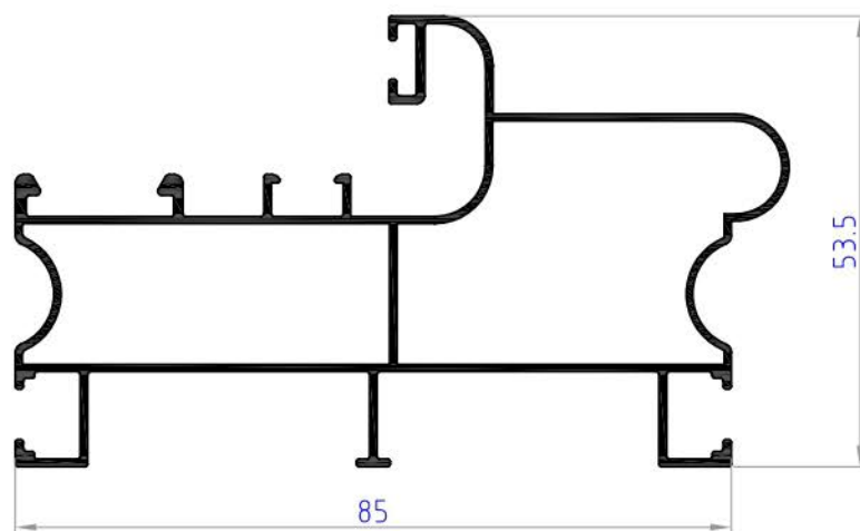
PS5606 weight 0.892 kg/ml
