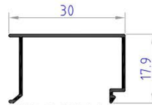
NC1374 weight 0.149 kg/ml
