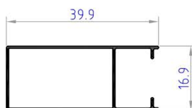
NC5504 weight 0.252 kg/ml
