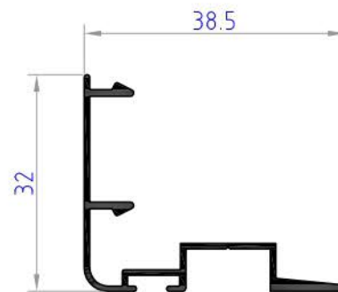
PS6603 weight 0.253 kg/ml
