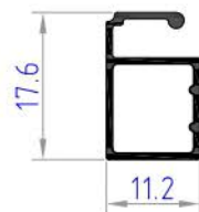
NC1517 weight 0.145 kg/ml
