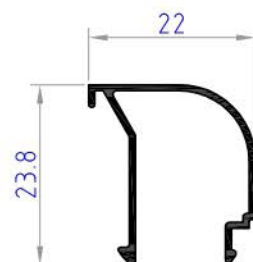
PS4812 weight 0.157 kg/ml
