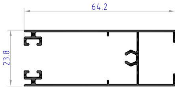
NC1216 weight 0.538 kg/ml
