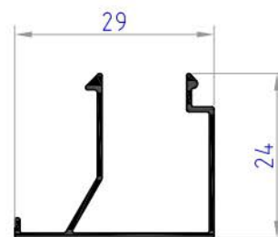
PS5611 weight 0.167 kg/ml
