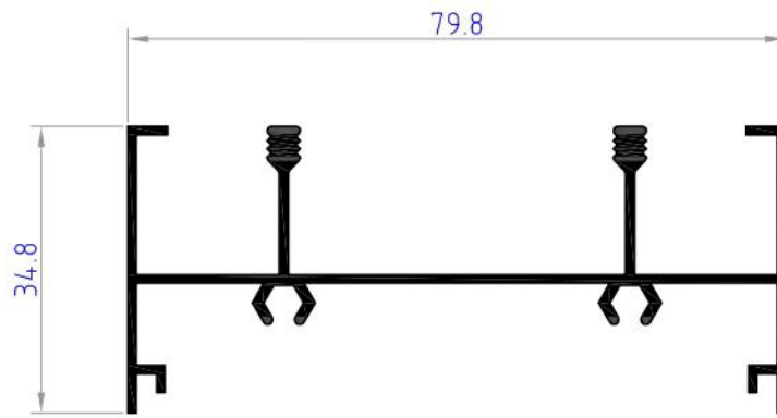
NC1227 weight 0.630 kg/ml
