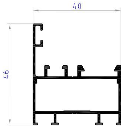
PS4805 weight 0.432 kg/ml
