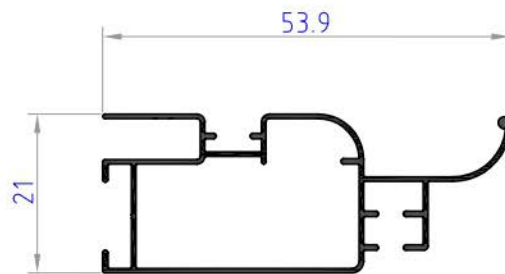
PS6006 weight 0.368 kg/ml
