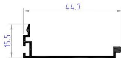
NC1285 weight 0.168 kg/ml
