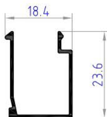
PS5613 weight 0.147 kg/ml
