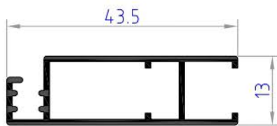
NC1515 weight 0.258 kg/ml
