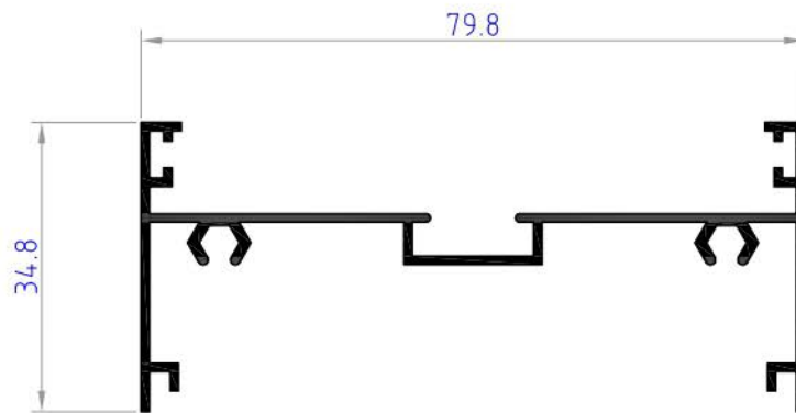
NC1228 weight 0.540 kg/ml
