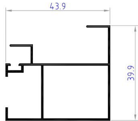
NC1219 weight 0.379 kg/ml
