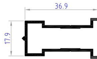
AM116 weight 0.240 kg/ml
