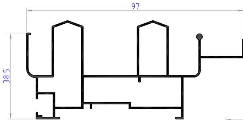
PS6622 weight 0.780 kg/ml
