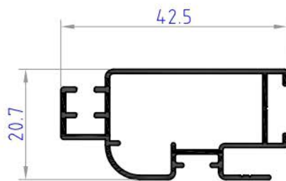
PS6606 weight 0.322 kg/ml
