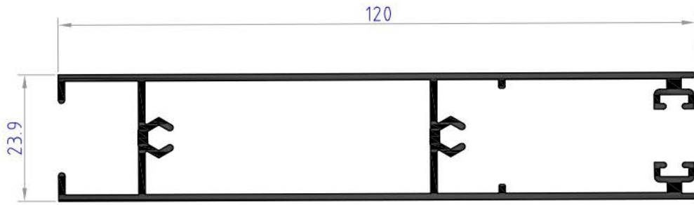
NC1215 weight 0.950 kg/ml
