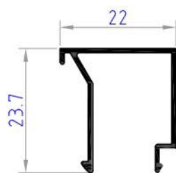
PS4811 weight 0.160 kg/ml
