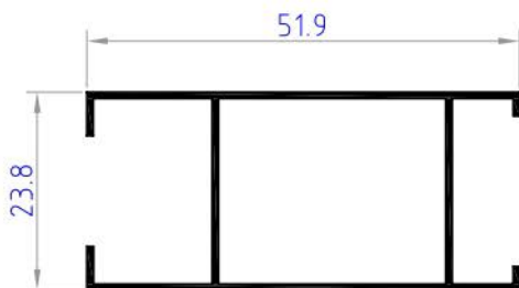
NC1221 weight 0.314 kg/ml
