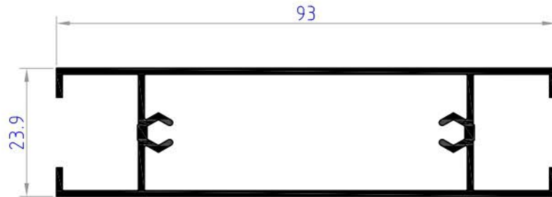
NC1210 weight 0.619 kg/ml
