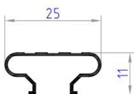
MY02 weight 0.096 kg/ml
