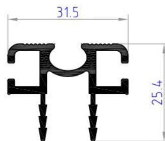
TRN 01 weight 0.538 kg/ml
