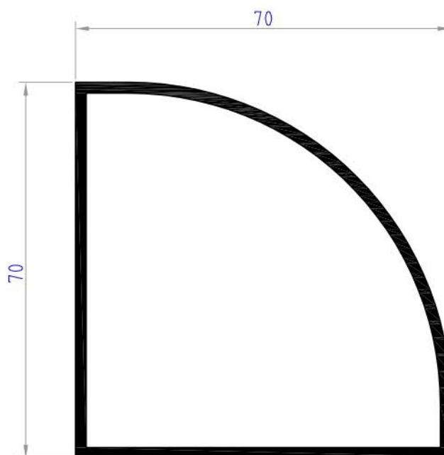
CH01 weight 1.293 kg/ml
