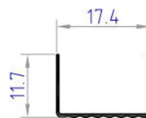
ST6016B weight 0.065 kg/ml
