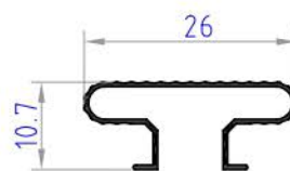
MY03 weight 0.085 kg/ml
