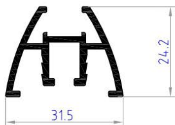
TRN 02 weight 0.368 kg/ml
