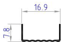
MSD01 weight 0.049 kg/ml
