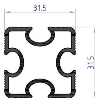
TRN 03 weight 0.473 kg/ml
