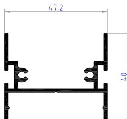
TRN 09 weight 0.665 kg/ml
