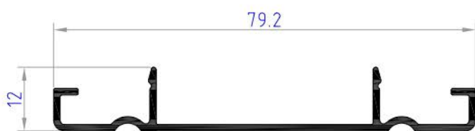
TRN 04 weight 0.391 kg/ml
