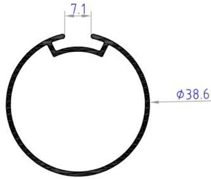
NMK38 weight 0.328 kg/m
