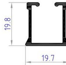
CUR01 weight 0.208 kg/m
