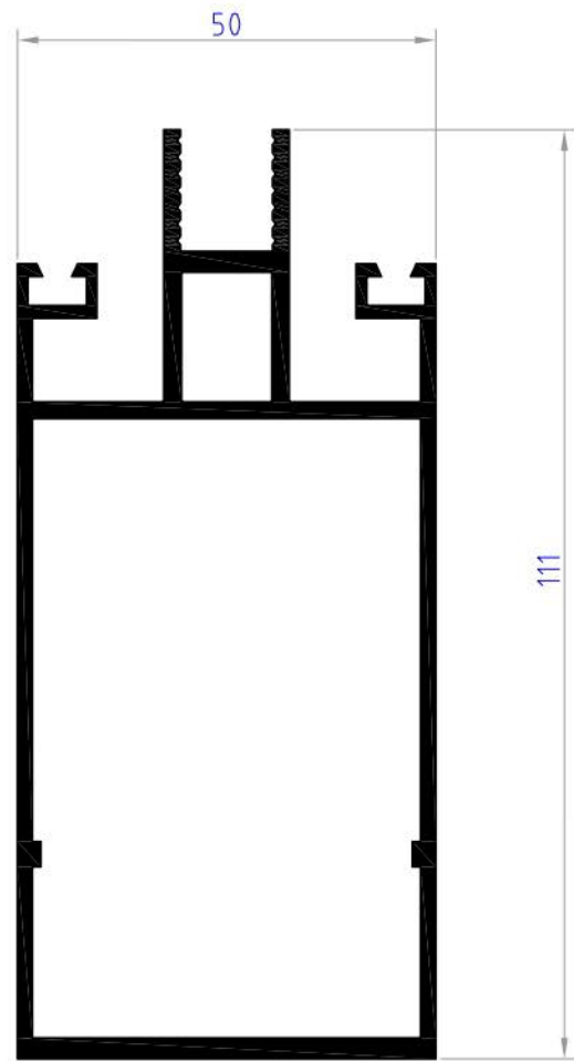
CP02 weight 1.896 kg/ml
