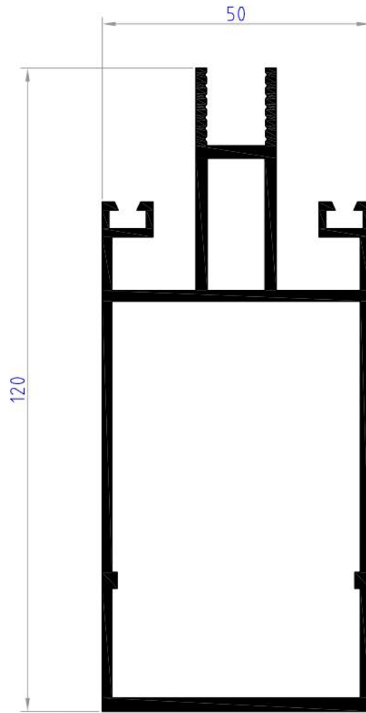
CP04 weight 1.955 kg/ml
