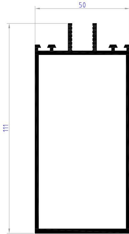
CP01 weight 1.565 kg/ml
